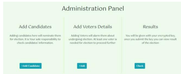
Figure 4. Admin panel.
