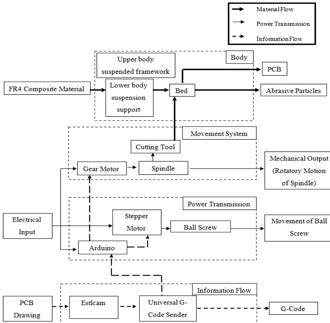
Figure 4. Cluster Function Structure for CNC PCB Plotter.
